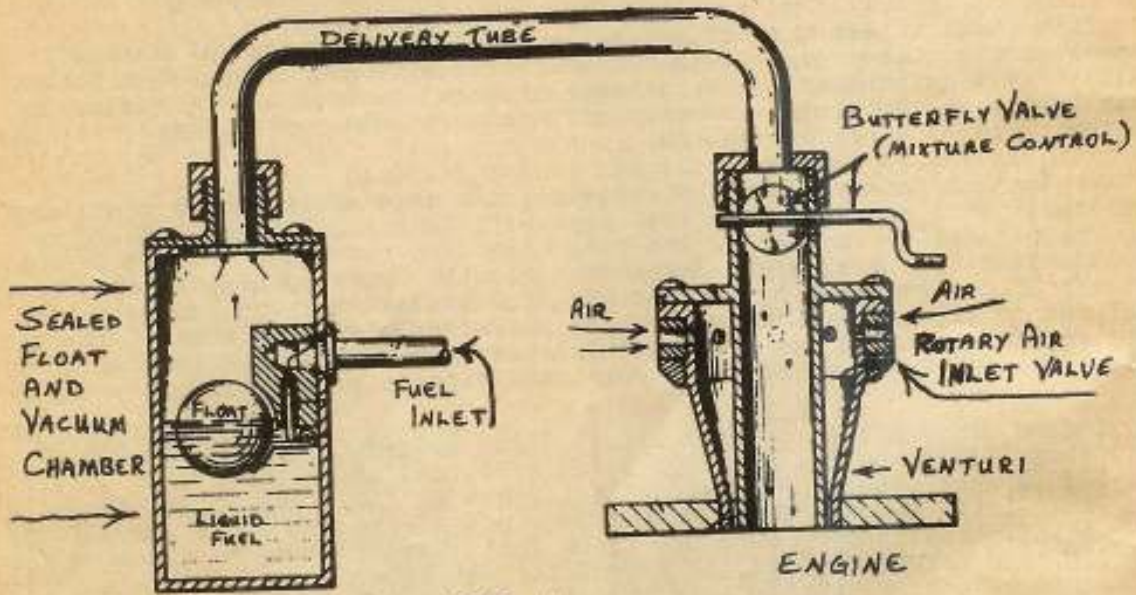
FIG. 1 SIDE VIEW
